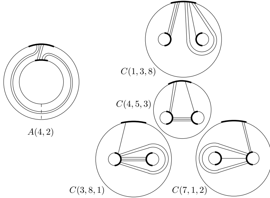
Figure 2: Examples of elementary multicurves
