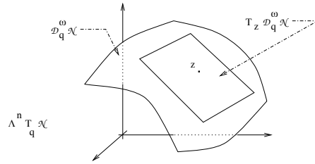
Figure 2: T_z D_q^\omega \mathcal{N} is a vector subspace of \Lambda^n T_q \mathcal{N}
