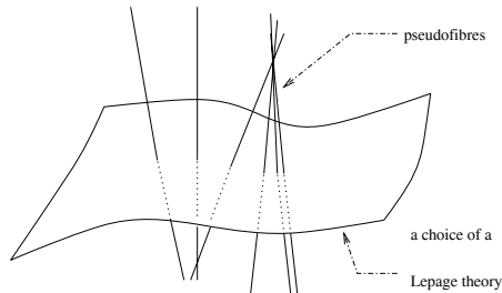
Figure 1: Pseudofibers which intersect a submanifold corresponding to the choice of a Lepage theory
