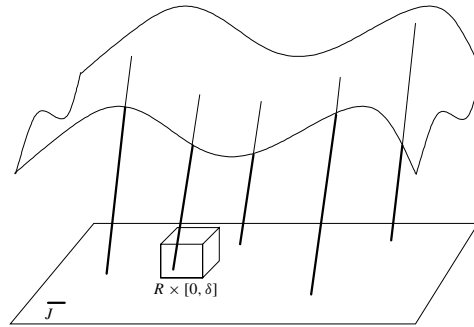
FIGURE 1. An interval J and its image.
